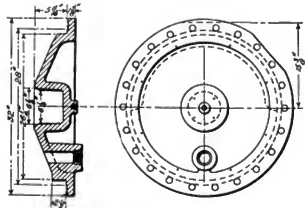
Figs. 926-927. Front Head. Cylinder Heads, Consolidation (2-8-0) Locomotive. American Locomotive Co.
